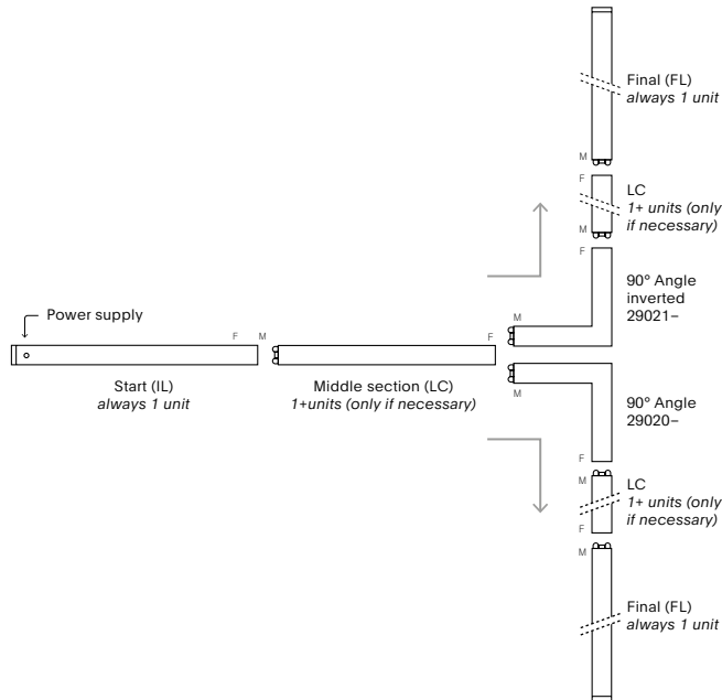
L-shaped structure
