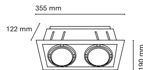
Cut-out 165x327mm
