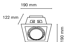
Cut-out 165x165mm
