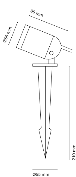
24806- Far Spike 55
