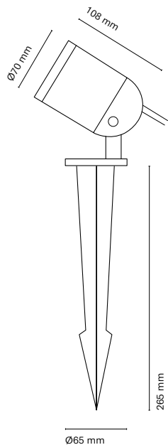
24807- Far Spike 70
