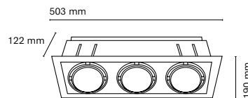
Cut-out 165x472mm
