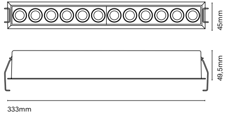
24622- Vlok Recessed
