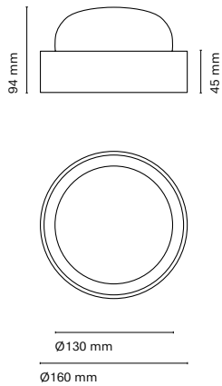
24511- Sight round
