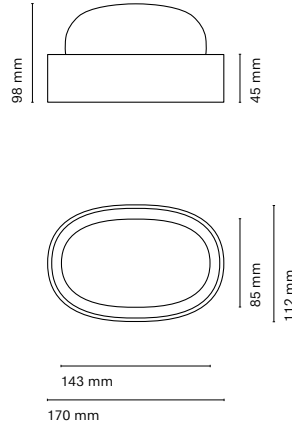
24521- Sight oval
