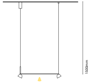
31512- Aros Single
